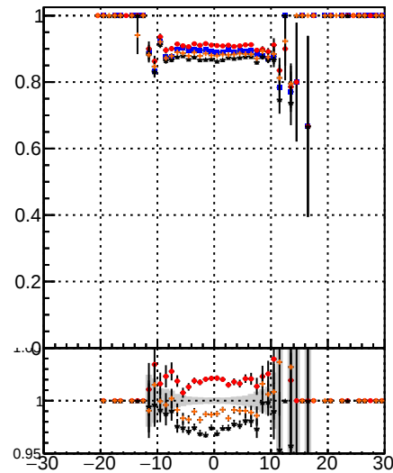
Fake rate vs v DOM IT CKE DOM IT CKEfit DOM IT BDT DOM IT mkFit
