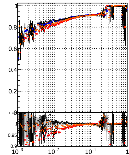
Legend for Fake rate vs dr: DOM (black line) IT (blue line) CKE (red line) BDT (orange line) DOM (black line) IT (blue line) CKE (red line) BDT (orange line) DOM (black line) IT (blue line) CKE (red line) BDT (orange line)
