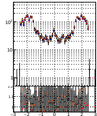
N of reco track vs \eta Legend: BQM (black), TT (blue), CKEfit (red), BDT (orange)
