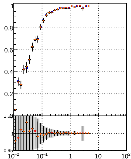
Fake rate vs v DOM IT CKE DOM IT CKE fit DOM IT BDT DOM IT CKE fit BDT
