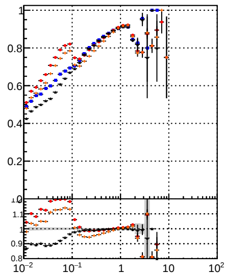
Fake rate vs v DOM TT CKE CKE fit BDT BDT fit
