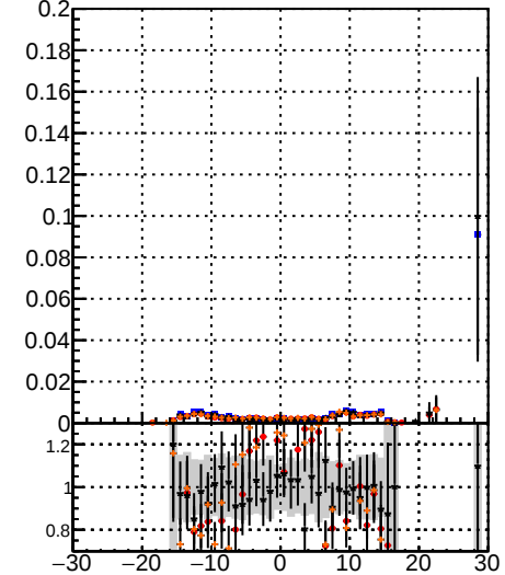
Duplicates Rate vs v DOM TT CKE CKE fit BDT BDT fit
