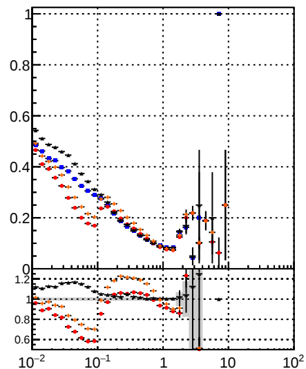
Pileup rate vs v DOM TT CKE CKE fit BDT BDT fit
