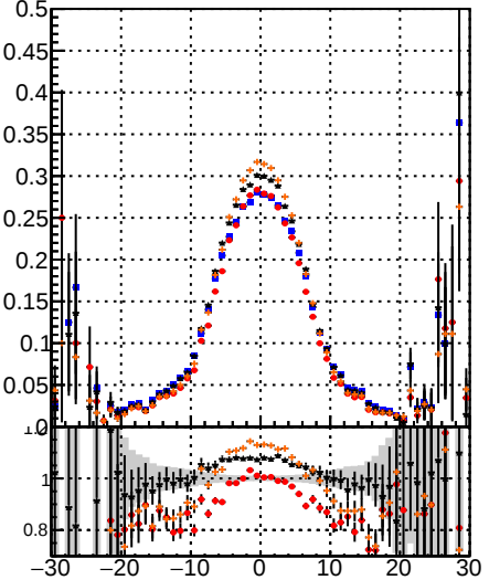
Pileup rate vs v DOM TT CKE CKE fit BDT BDT fit
