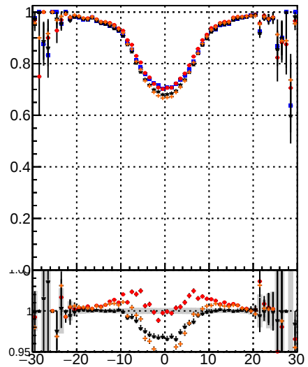
Fake rate vs v DOM TT CKE CKE fit BDT BDT fit
