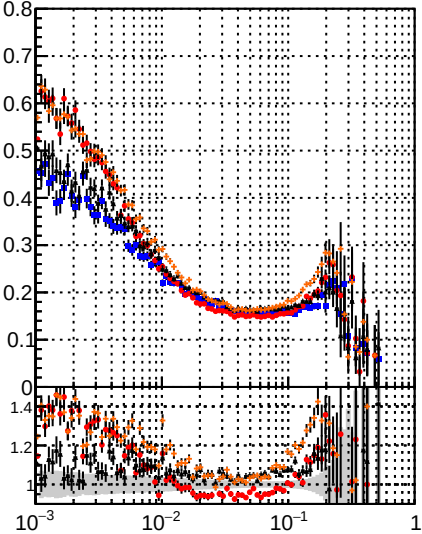
Pileup rate vs \epsilon
