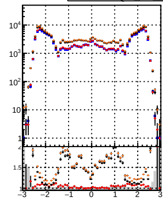
N of reco track vs \eta Legend: BQM, CKFit, BDT, CKFit, BDT, CKFit, BDT
