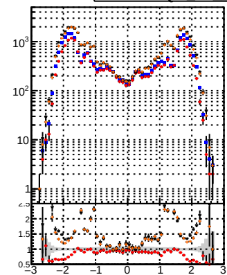
N of reco track vs \eta Legend: BQM, CKFit, BDT
