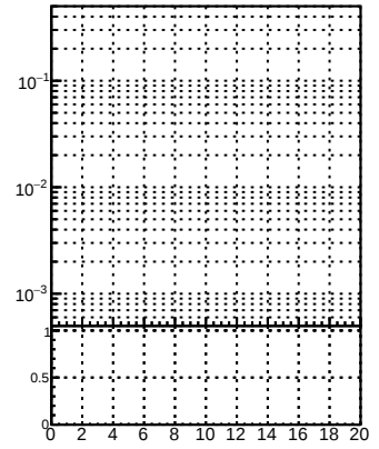
N of associated (recoToSim) loopier tracks vs normalized \chi^2
