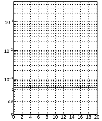
N of reco track vs normalized \chi^2
