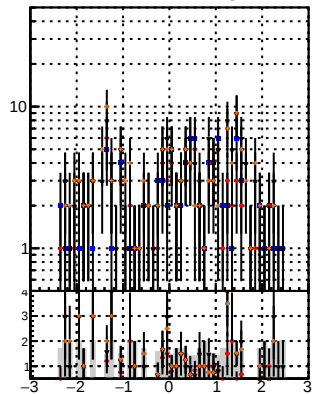
N of reco track vs \eta Legend: BQM (black), TT (blue), CKEFit (red), mkrFit (orange)
