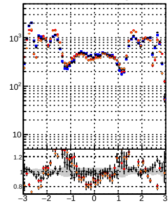
N of reco track vs \eta Legend: BQM (black), TT (blue), CKFit (red), mkrFit (orange)
