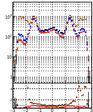
N of reco track vs \eta Legend: BQM (blue), CKFit (orange), BDT (red), BQM (black), CKFit (black), BDT (black)
