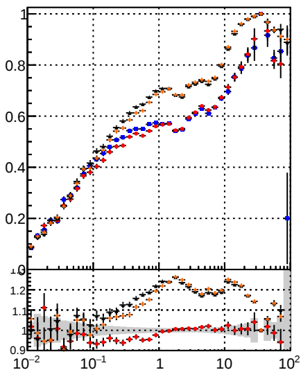
Legend for Fake rate vs v: DOM CKE CKEfit BDT BDTfit
