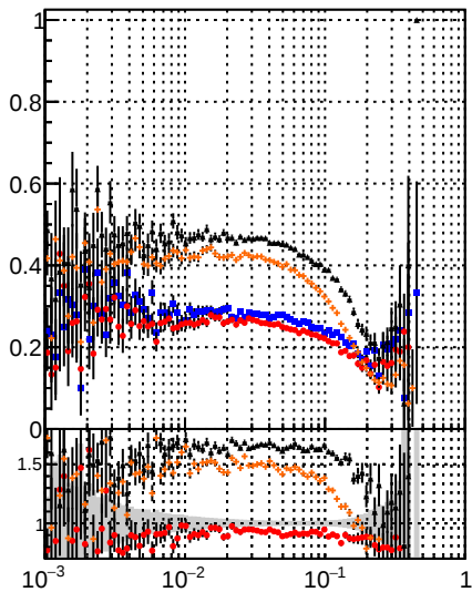
Fake rate vs \epsilon Legend: DOM TT CKE DOM TT CKE fit DOM TT mktFit BDT
