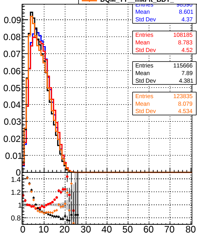
— DQM_TT_CKF_ (Blue) — DQM_TT_mkFit_ (Red) — DQM_TT_CKF_BDT_ (Black) — DQM_TT_mkFit_BDT_ (Orange)
