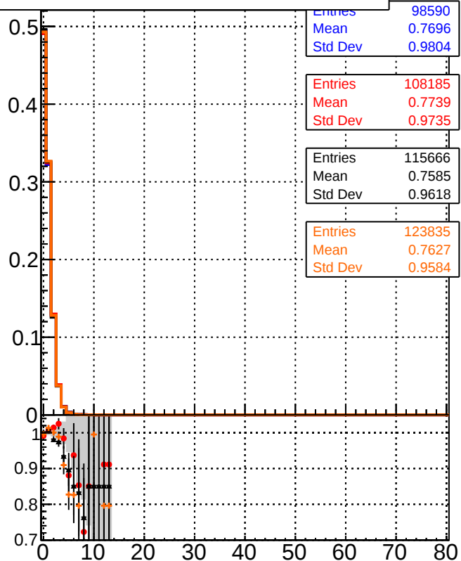
— DQM_TT_CKF_ (Blue) — DQM_TT_mkFit_ (Red) — DQM_TT_CKF_BDT_ (Black) — DQM_TT_mkFit_BDT_ (Orange)
