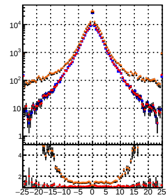
—●— DOM TT CKE mkFit BDT —●— DOM TT CKE mkFit BDT —●— DOM TT CKE mkFit BDT
