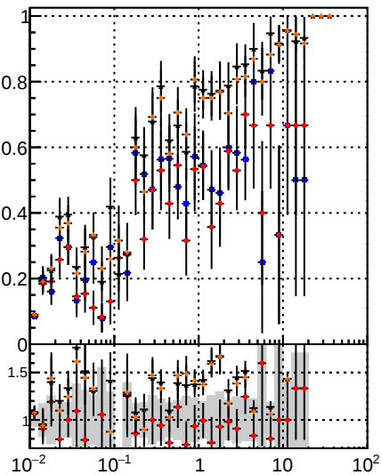
Fake rate vs v DOM TT CKE DOM TT CKE fit DOM TT mktFit DOM TT BDT
