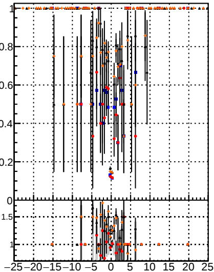
Fake rate vs d BSM CKFit BDT BSM CKFit BDT
