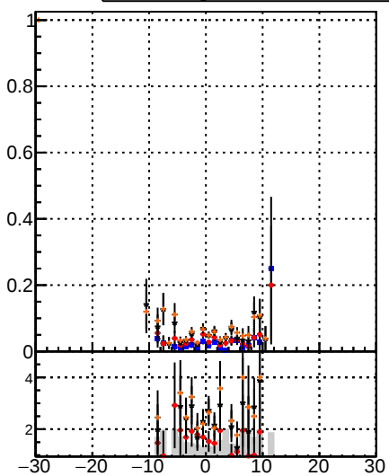
Fake rate vs v_z Legend: DOM IT CKE DOM IT CKE DOM IT mktFit BDT
