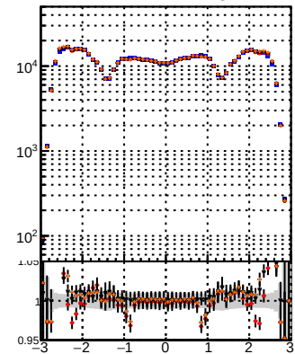
N of reco track vs \eta Legend: BQM, TT, CKEFit, BDT
