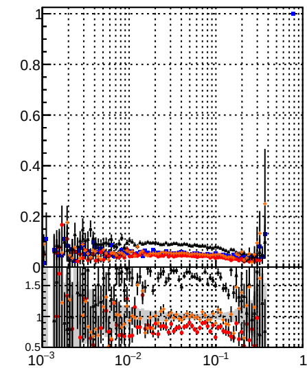
Fake rate vs \epsilon Method Symbol Line Style DOM Black circle Solid IT Blue square Solid CKE Red triangle Solid BDT Orange diamond Solid DOM Black circle Dashed IT Blue square Dashed CKE Red triangle Dashed BDT Orange diamond Dashed DOM Black circle Dotted IT Blue square Dotted CKE Red triangle Dotted BDT Orange diamond Dotted
