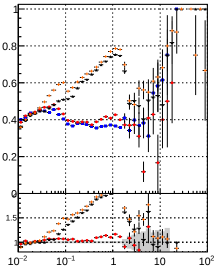
Fake rate vs \nu Method Symbol DOM Blue circle IT Orange cross CKE Black dot CKE fit Red dot BDT Grey square mke fit Black dot
