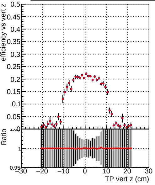
Efficiency vs TP vert z (cm) Legend: DQM_TT_ORIGINAL (grey histogram) DQM_TT_MODIFIED_propToPlane_PRRVersionFINAL6 (red line with error bars)
