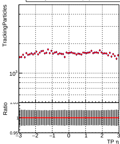
N of simulated tracks vs \eta Legend: — DQM_TT_ORIGINAL (blue line with dots) — DQM_TT_MODIFIED_propToPlane_PRVersionFINAL6 (red line with stars)
