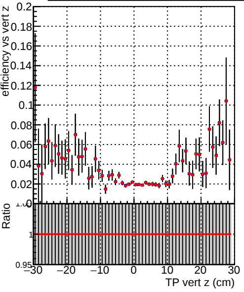
Efficiency vs TP vert z (cm) Legend: DQM_TT_ORIGINAL (blue line), DQM_TT_MODIFIED_propToPlane_PRRVersionFINAL6 (red line)
