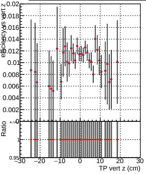
Efficiency vs TP vert z (cm) Legend: DQM_TT_ORIGINAL (Blue line with markers) DQM_TT_MODIFIED_propToPlane_PRRVersionFINAL6 (Red line with markers)
