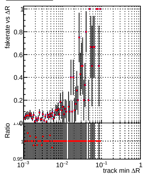
Fake rate vs —•— DQM_TT_ORIGINAL —•— DQM_TT_MODIFIED_propToPlane_PRVersionFINAL6
