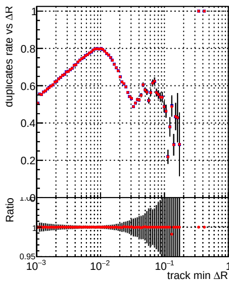
—•— DQM_TT_ORIGINAL —•— DQM_TT_MODIFIED_propToPlane_PRVersionFINAL6
