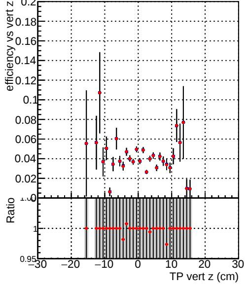
Efficiency vs. TP vert z Legend: DQM_TT_ORIGINAL (blue line), DQM_TT_MODIFIED_propToPlane_PRVersionFINAL6 (red line)
