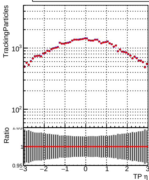
N of simulated tracks vs TP \eta Legend: DQM_TT_ORIGINAL (blue line with dots), DQM_TT_MODIFIED_propToPlane_PRVersionFINAL6 (red line with dots)
