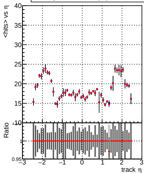
mean hits Legend: DQM_TT_ORIGINAL (blue line with markers), DQM_TT_MODIFIED_propToPlane_PRVersionFINAL6 (red line with markers)
