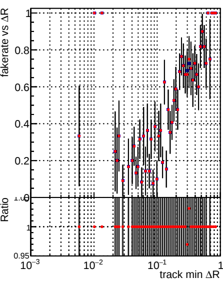
Legend: DQM_TT_ORIGINAL (grey bars), DQM_TT_MODIFIED_propToPlane_PRVersionFINAL6 (red dots with error bars)
