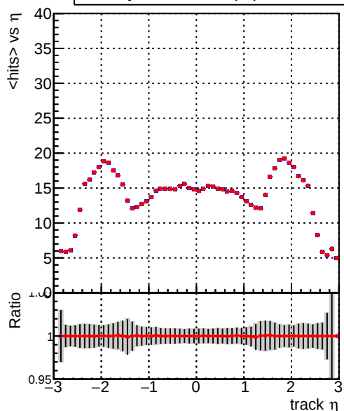
mean hits vs \eta Legend: DQM_TT_ORIGINAL (blue line), DQM_TT_MODIFIED_propToPlane_PRVersionFINAL6 (red line)
