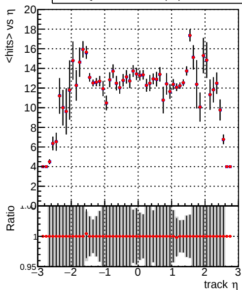
mean hit — DQM_TT_ORIGINAL — DQM_TT_MODIFIED_propToPlane_PRVersionFINAL6
