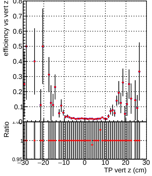
Efficiency vs vert z Legend: — DQM_TT_ORIGINAL — DQM_TT_MODIFIED_propToPlane_PRRVersionFINAL6
