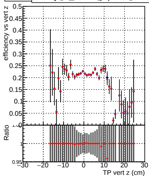
Efficiency vs. TP vert z (cm) — DQM_TT_ORIGINAL — DQM_TT_MODIFIED_propToPlane_PRRVersionFINAL6
