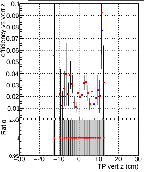
Efficiency vs vertpos Legend: DQM_TT_ORIGINAL DQM_TT_MODIFIED_propToPlane_PRRVersionFINAL6
