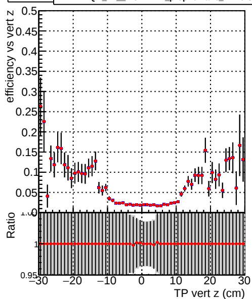
Efficiency vs TP vert z — DQM_TT_ORIGINAL — DQM_TT_MODIFIED_propToPlane_PRVersionFINAL6
