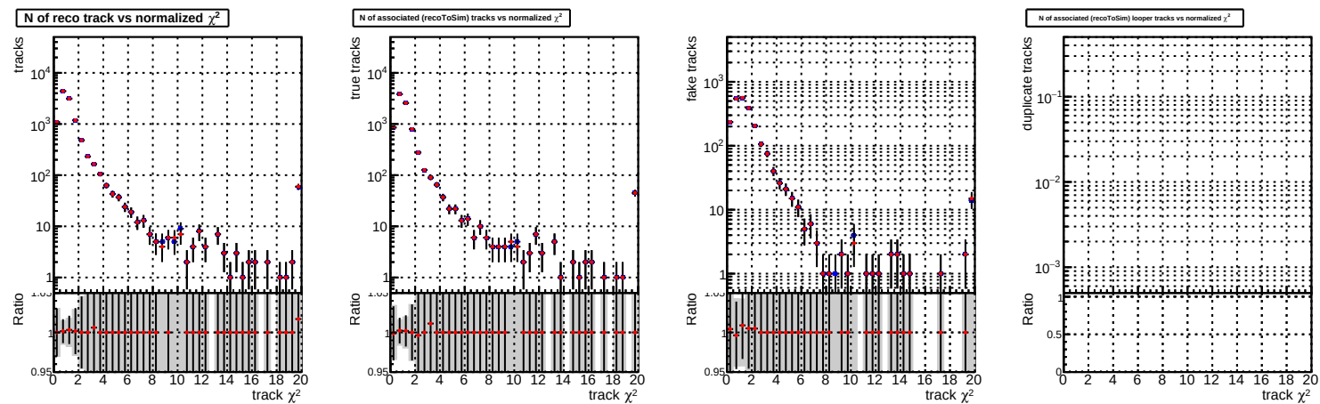
N of reco track vs. \chi^2 Legend: DOM TT ORIGINAL (blue circles) DOM TT MODIFIED_propToPlane_PVersionFINAL6 (red circles)
