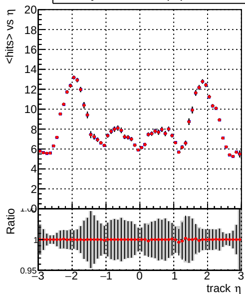
mean hits Legend: DQM_TT_ORIGINAL (blue line), DQM_TT_MODIFIED_propToPlane_PRVersionFINAL6 (red line)
