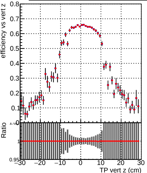
Efficiency vs TP vert z (cm) Legend: DQM_TT_ORIGINAL DQM_TT_MODIFIED_propToPlane_PRRVersionFINAL5
