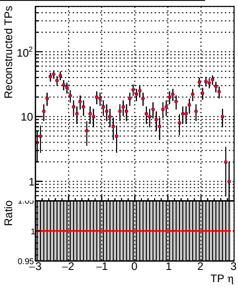
Legend: DQM_TT_ORIGINAL (blue line with dots), DQM_TT_MODIFIED_propToPlane_PRVersionFINAL5 (red line with dots)
