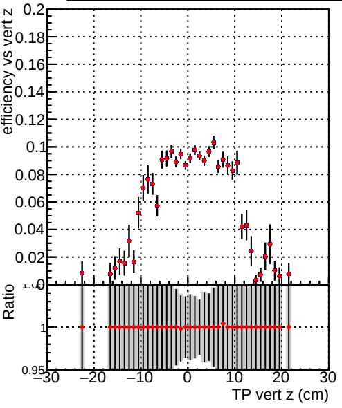
Efficiency vs TP vert z (cm) Legend: DQM_TT_ORIGINAL DQM_TT_MODIFIED_propToPlane_PRRVersionFINAL5
