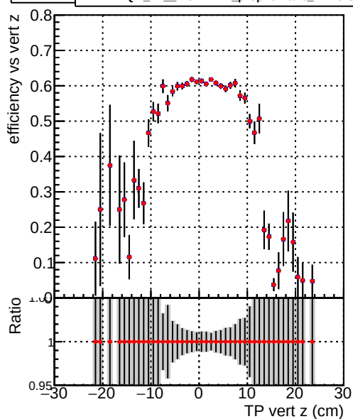
Efficiency vs. TP vert z (cm) — DQM_TT_ORIGINAL — DQM_TT_MODIFIED_propToPlane_PRVersionFINAL5
