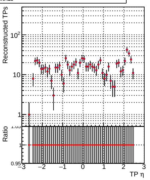
N of associated tracks (simToReco) vs \eta
