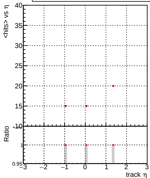
mean hits vs \eta Legend: DQM_TT_ORIGINAL (blue line with dots), DQM_TT_MODIFIED_propToPlane_PRVersionFINAL5 (red line with dots)
