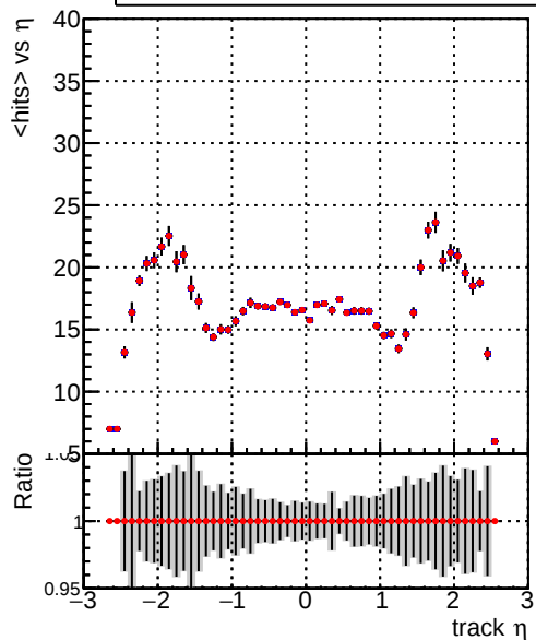
mean hits Legend: DQM_TT_ORIGINAL (blue line), DQM_TT_MODIFIED_propToPlane_PRVersionFINAL5 (red line)
