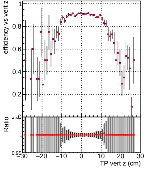
Efficiency vs TP vert z Legend: DQM_TT_ORIGINAL (blue line), DQM_TT_MODIFIED_propToPlane_PRVersionFINAL5 (red line)
