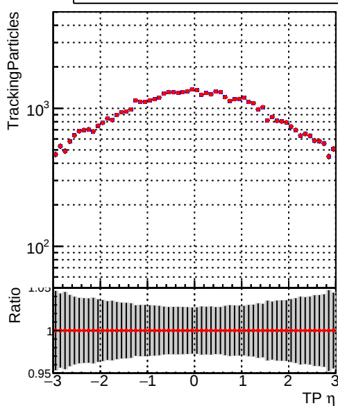
N of simulated tracks vs TP \eta Legend: DQM_TT_ORIGINAL (blue line), DQM_TT_MODIFIED_propToPlane_PRVersionFINAL5 (red line)
