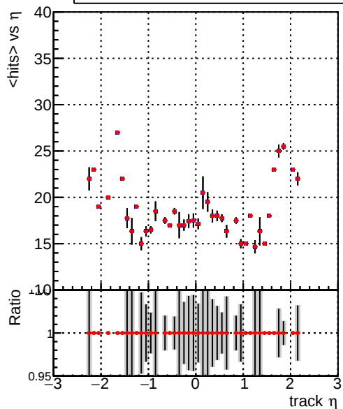
mean hits vs \eta — DQM_TT_ORIGINAL — DQM_TT_MODIFIED_propToPlane_PRVersionFINAL5
